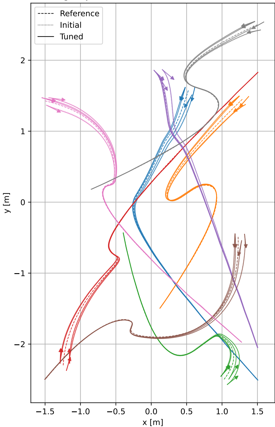
Training Trajectories (8 shown, 4 start offsets each)
